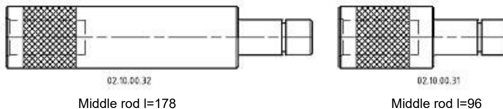
Rods for working tools
